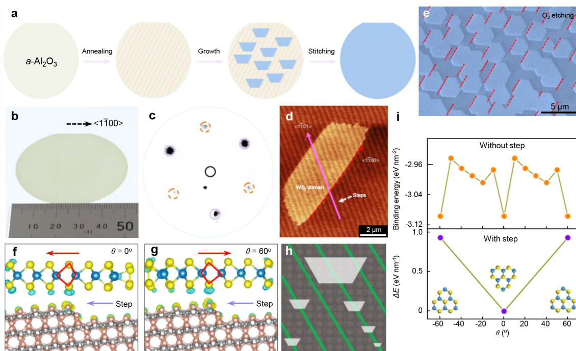
Figure 13. (a) The growth process of single-crystal \text{WS}_2 films on \text{a-Al}_2\text{O}_3 . (b) A photograph of \text{WS}_2/\text{a-Al}_2\text{O}_3 . (c) Representative LEED pattern of the \text{WS}_2 film. (d) AFM image of a \text{WS}_2 island. (e) False-color SEM image of \text{WS}_2 films after \text{O}_2 etching. (f,g) Optimized structures of antiparallel \text{WS}_2 on \text{a-Al}_2\text{O}_3 . (h) Schematic of \text{WS}_2 islands grown on \text{a-Al}_2\text{O}_3 during the early stage of growth. (i) Theoretical analysis and DFT calculation of \text{WS}_2 epitaxial growth with and without steps. (Reproduced from ref 61. Copyright 2022 Springer Nature).
