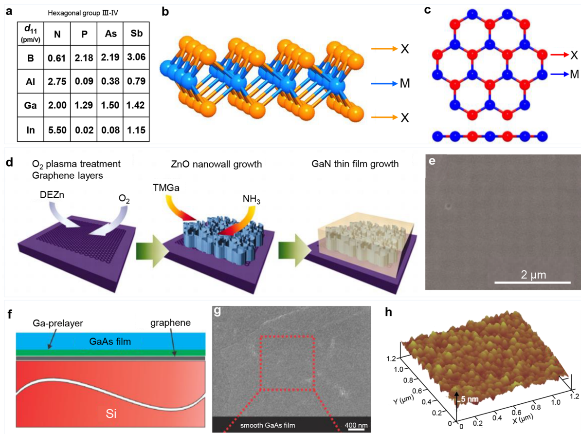
Figure 22. (a) Periodic trends for d_{11} in group III–V semiconductors. (b,c) 2D and planar hexagonal structures of group III–V semiconductors. (Reproduced from ref 207. Copyright 2015 American Chemical Society). (d) Schematic diagrams of epitaxial growth of GaN thin films. (e) GaN thin film grown on ZnO nanowalls. (Reproduced from ref 212. Copyright 2010 American Association for the Advancement of Science). (f) Schematic diagram of cross-section view of the GaAs films/Ga-prelayer/graphene/Si. (g) SEM plan-view image and (h) AFM image of ultrasmooth GaAs films. (Reproduced from ref 213. Copyright 2014 Wiley).
