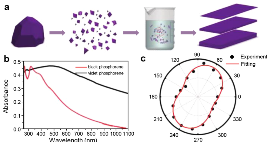
Figure 19. (a) The preparation processes, (b) UV–vis–NIR absorption spectrum of violet phosphorene. (c) The angle-dependent SHG polarization pattern. (Reproduced from ref 185. Copyright 2023 Wiley).
