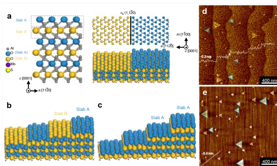
Figure 14. (a–c) Schematic diagrams of sapphire surface with 3-fold atomic arrangement. (d,e) AFM images of antiparallel and unidirectional aligned \text{MoS}_2 islands. (Reproduced from ref 55. Copyright 2023 Springer Nature).
